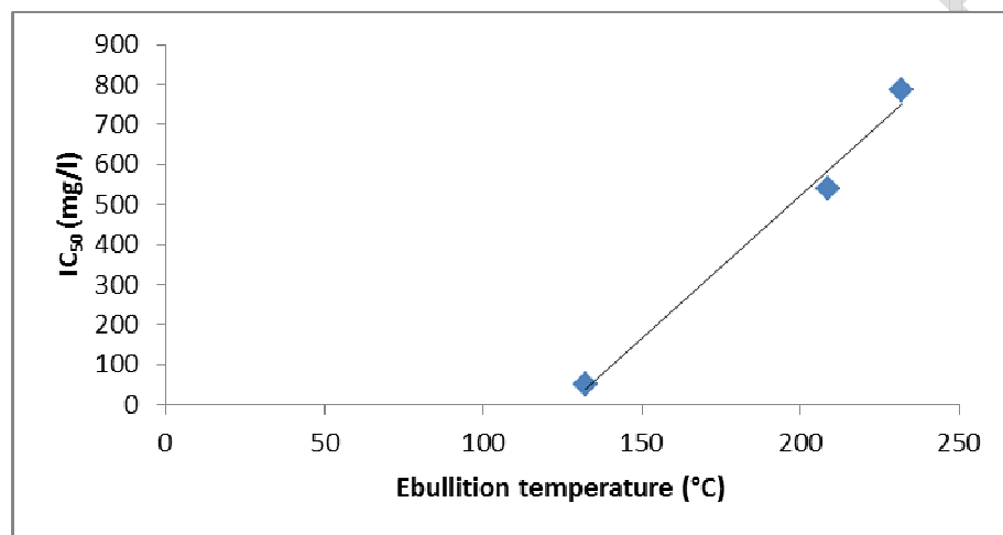
Fig. 4: Methanogenic toxicity ( IC_{50} ) with Chloroaniline isomers boiling point correlation ( R^2 = 0.989 ).
